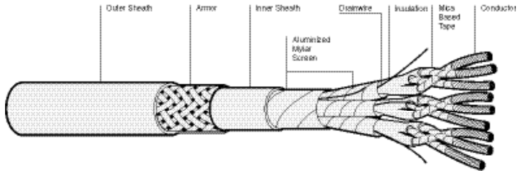
FR-1000 multitriple control cables, Collectively Shielded and Armored, 600/1000V*
