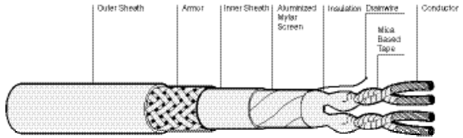
FR-1000 Multipair Control Cables, Collectively Shielded and Armored 600/1000V*
