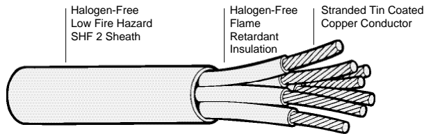
SeaLite SL105-SU Multicore Unshielded Cables
