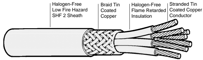
SeaLite SL105-SO Multicore Overall Shielded Cables
