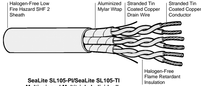
SeaLite SL105-PI/SeaLite SL105-TI Multipair and Multitriples Individually Shielded Cables
