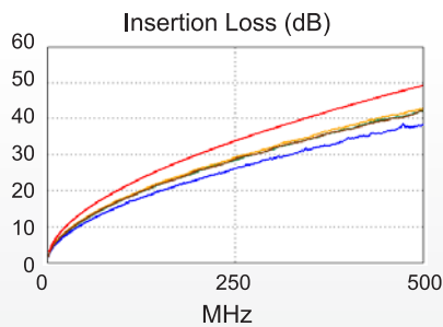
Figure 5: E6A6824 Insertion Loss
