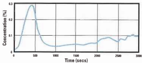
LSZH (IEC 332-1) in Full-Scale Carbon Monoxide Tests at BRE/FRS
