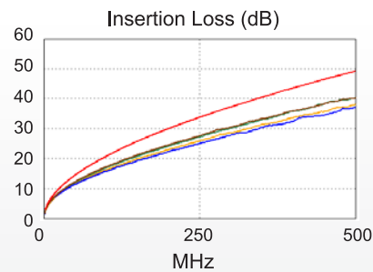
Figure 6: E6A6826 Insertion Loss
