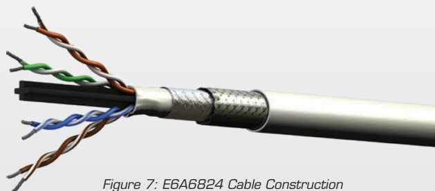
Figure 7: E6A6824 Cable Construction
