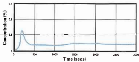
CMP Cable in Full-Scale Carbon Monoxide Tests at BRE/FRS
