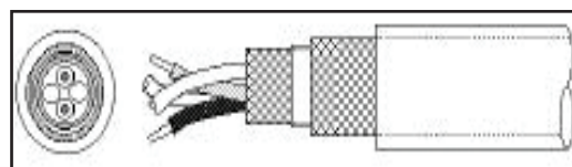
Figure 2. Quadaxial cable design.
