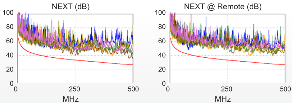
Figure 2: E6A6824 Near End Cross Talk (NEXT)
