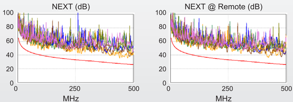
Figure 3: E6A6826 Near End Cross Talk (NEXT)
